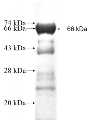
Recombinant Human RAB3IL1 SDS-PAGE
