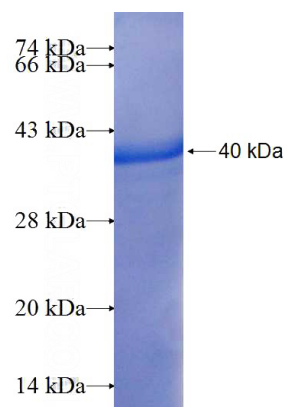
Recombinant Human FOSL1 SDS-PAGE
