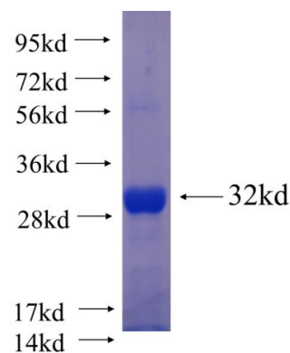
Recombinant human HECTD3 SDS-PAGE
