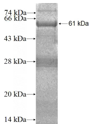
Recombinant Human A4GALT SDS-PAGE
