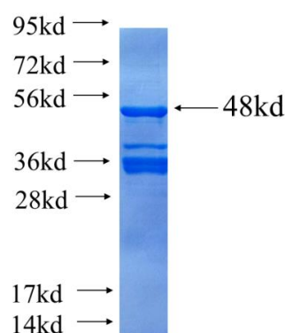
Recombinant human SSX4(Full length) SDS-PAGE
