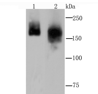
Fig1: Western blot analysis of Clathrin heavy chain on Hela (1) and PC-12 (2) cell lysate using anti-Clathrin heavy chain antibody at 1/1,000 dilution.
