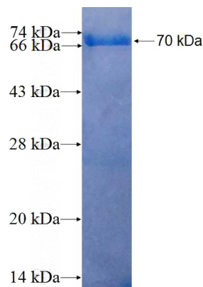
Recombinant Human KRT19 SDS-PAGE
