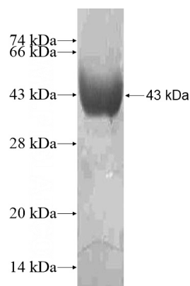
Recombinant Human PPP1R10 SDS-PAGE
