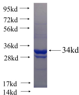
Recombinant human SLC22A6 SDS-PAGE
