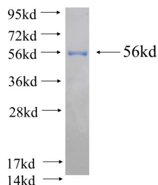
Recombinant human IFT52(Full length) SDS-PAGE
