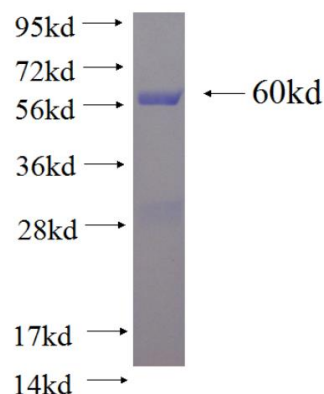
Recombinant human KMO SDS-PAGE
