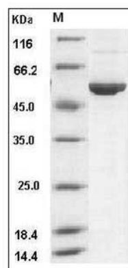
Human ALDH3A1 Protein (His Tag) SDS-PAGE
