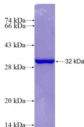
Recombinant Human FASN SDS-PAGE
