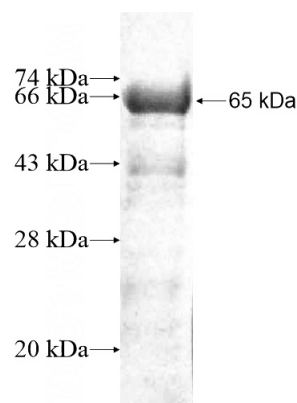
Recombinant Human LUZP1 SDS-PAGE
