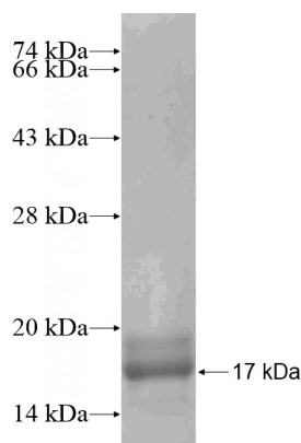
Recombinant Human TMEM185A SDS-PAGE
