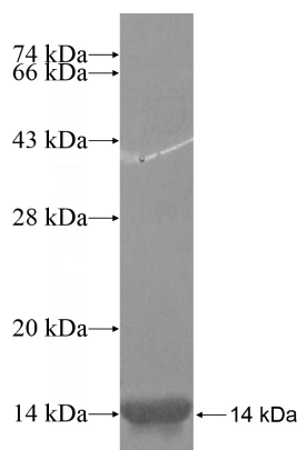
Recombinant Human SLC17A4 SDS-PAGE
