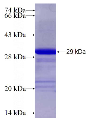
Recombinant Human PHKA1 SDS-PAGE
