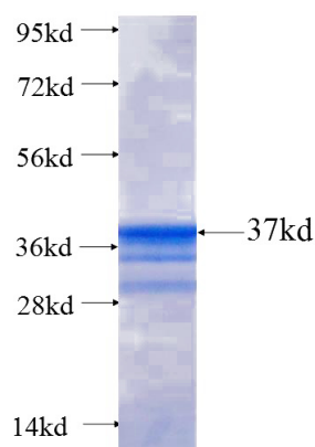
Recombinant Human TERT SDS-PAGE
