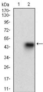
Western blot analysis using PRL mAb against HEK293 (1) and PRL (AA
