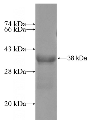
Recombinant Human BTBD10 SDS-PAGE
