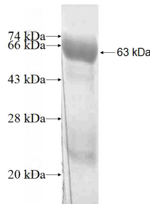
Recombinant Human RPIA SDS-PAGE
