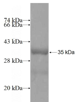
Recombinant Human MRPL10 SDS-PAGE
