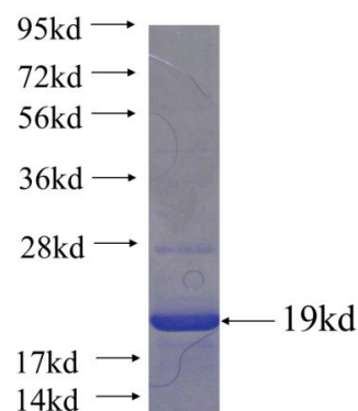
Recombinant human CCK SDS-PAGE
