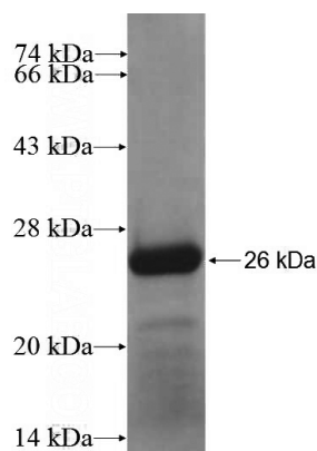
Recombinant Human ADAMTS18 SDS-PAGE
