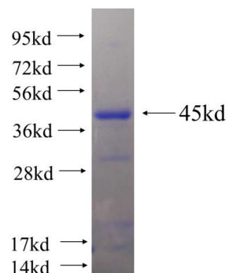
Recombinant human EIF4G1 SDS-PAGE
