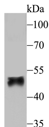
Fig1: Western blot analysis of FOXF2 on human placenta tissue lysate using anti-FOXF2 antibody at 1/200 dilution.
