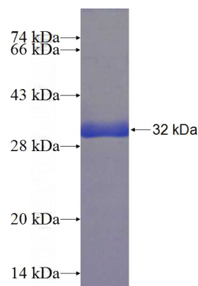
Recombinant Human A1CF SDS-PAGE
