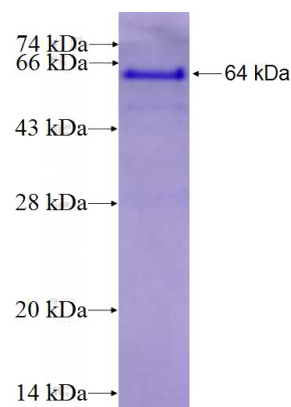
Recombinant Human RIC8A SDS-PAGE
