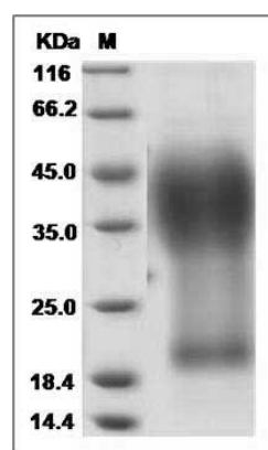
Human GYPA / CD235a / Glycophorin A Protein (His Tag) SDS-PAGE
