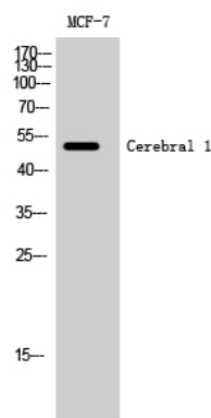
Fig1.; Western Blot analysis of MCF-7 cells using Cerebral 1 Polyclonal Antibody cells nucleus extracted by Minute TM Cytoplasmic and Nuclear Fractionation kit (SC-003, Inventibiotec, MN, USA).
