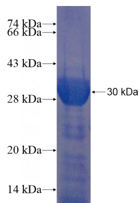
Recombinant Human PACRGL SDS-PAGE
