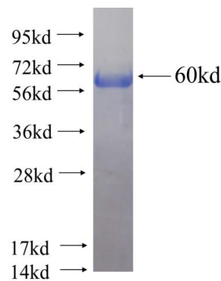
Recombinant human ARPC2(Full length) SDS-PAGE
