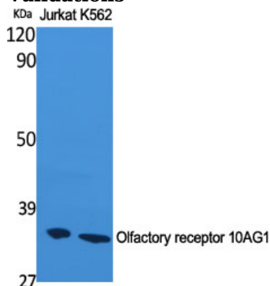
Fig1.: Western Blot analysis of various cells using Olfactory receptor 10AG1 Polyclonal Antibody
