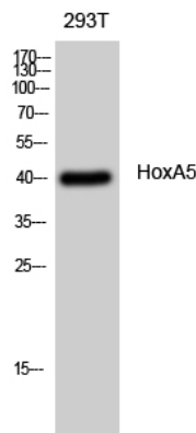
Fig1;; Western Blot analysis of 293T cells using HoxA5 Polyclonal Antibody diluted at 1: 500 cells nucleus extracted by Minute TM Cytoplasmic and Nuclear Fractionation kit (SC-003, Inventbiotech, MN, USA).
