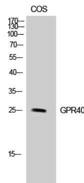
Fig1.: Western Blot analysis of COS7 cells using GPR40 Polyclonal Antibody diluted at 1: 500
