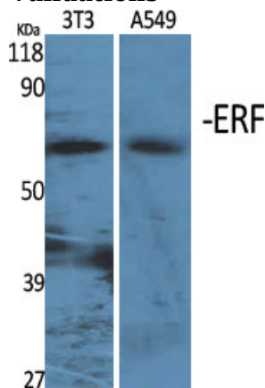
Fig1.; Western Blot analysis of various cells using ERF Polyclonal Antibody cells nucleus extracted by Minute TM Cytoplasmic and Nuclear Fractionation kit (SC-003, Inventbiotech, MN, USA).
