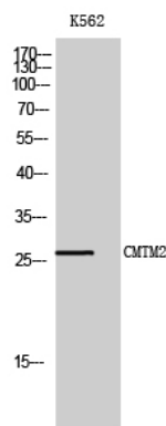
Fig1.; Western Blot analysis of K562 cells using CMTM2 Polyclonal Antibody
