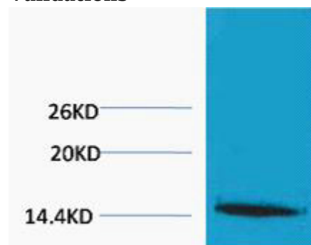
Fig1:; Western blot analysis of extracts from HeLa cells, 1:2000.. Secondary antibody (catalog#: HA1001) was diluted at 1:20000
