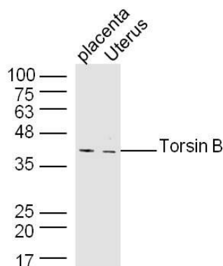
Fig1: Sample:; Placenta (Mouse) Lysate at 40 ug; Uterus (Mouse) Lysate at 40 ug; Primary: Anti-Torsin B at 1/300 dilution; Secondary: IRDye800CW Goat Anti-Rabbit IgG at 1/20000 dilution; Predicted band size: 36 kD; Observed band size: 40 kD
