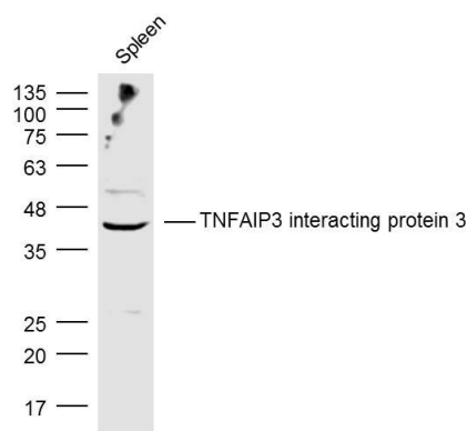
Fig1: Sample:; Spleen (Mouse) Lysate at 40 ug; Primary: Anti- TNFAIP3 interacting protein 3 at 1/300 dilution; Secondary: IRDye800CW Goat Anti-Rabbit IgG at 1/20000 dilution; Predicted band size: 39 kD; Observed band size: 39 kD
