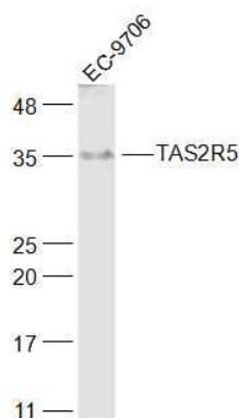
Fig1: Sample:; EC-9706(Human) Cell Lysate at 30 ug; Primary: Anti-TAS2R5 at 1/1000 dilution; Secondary: IRDye800CW Goat Anti-Rabbit IgG at 1/20000 dilution; Predicted band size: 34 kD; Observed band size: 35 kD
