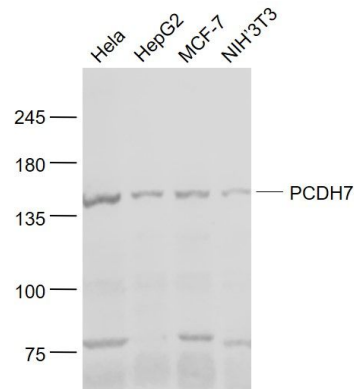
Fig1: Sample:; HeLa(Human) Cell Lysate at 30 ug; HepG2(Human) Cell Lysate at 30 ug; MCF-7(Human) Cell Lysate at 30 ug; NIH/3T3(Mouse) Cell Lysate at 30 ug; Primary: Anti- PCDH7 at 1/1000 dilution; Secondary: IRDye800CW Goat Anti-Rabbit IgG at 1/20000 dilution; Predicted band size: 113 kD; Observed band size: 150 kD
