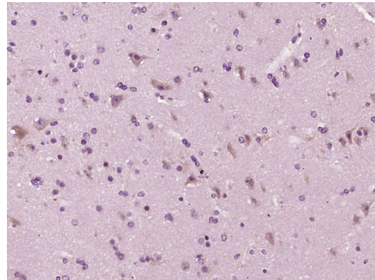
Fig2: Paraformaldehyde-fixed, paraffin embedded (HUMAN brain glioma); Antigen retrieval by boiling in sodium citrate buffer (pH6.0) for 15min; Block endogenous peroxidase by 3% hydrogen peroxide for 20 minutes; Blocking buffer (normal goat serum) at 37°C for 30min; Antibody incubation with (PCDH7) Polyclonal Antibody, Unconjugated at 1:400 overnight at 4°C, followed by operating according to SP Kit(Rabbit) (sp-0023) instructions and DAB staining.
