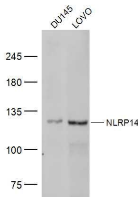
Fig1: Sample:; DU145(Human) Cell Lysate at 30 ug; LOVO(Human) Cell Lysate at 30 ug; Primary: Anti-NLRP14 at 1/300 dilution; Secondary: IRDye800CW Goat Anti-Rabbit IgG at 1/20000 dilution; Predicted band size: 125 kD; Observed band size: 125 kD
