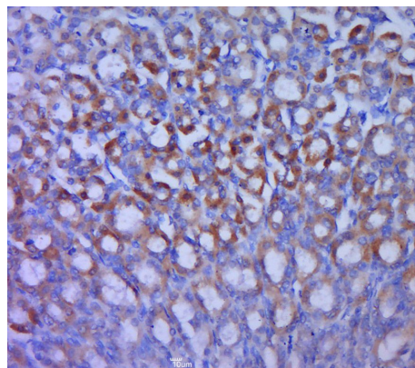
Fig1: Sample:; Heart (Rat) Lysate at 40 ug; Primary: Anti- GLUT12 at 1/300 dilution; Secondary: IRDye800CW Goat Anti-Rabbit IgG at 1/20000 dilution; Predicted band size: 68kD; Observed band size: 68kD
