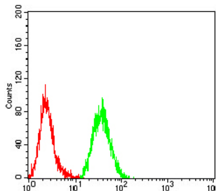
Fig4: Flow cytometric analysis of WDFY3 was done on HeLa cells. The cells were fixed, permeabilized and stained with the primary antibody ( 1/100) (green). After incubation of the primary antibody at room temperature for an hour, the cells were stained with a Alexa Fluor 488-conjugated goat anti-Mouse IgG Secondary antibody at 1/500 dilution for 30 minutes. Unlabelled sample was used as a control (cells without incubation with primary antibody; red).
