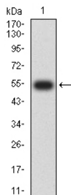
Fig1: Western blot analysis of WDFY3 against human WDFY3 (AA: 3277-3526) recombinant protein. Proteins were transferred to a PVDF membrane and blocked with 5% BSA in PBS for 1 hour at room temperature. The primary antibody (1/500) was used in 5% BSA at room temperature for 2 hours. Goat Anti-Mouse IgG - HRP Secondary Antibody at 1:5,000 dilution was used for 1 hour
