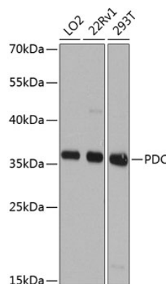
Western blot - PDC Polyclonal Antibody
