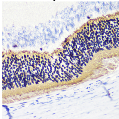
Immunohistochemistry - PDC Polyclonal Antibody
