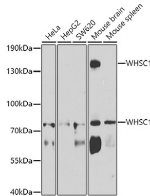
Western blot - WHSC1 Polyclonal Antibody
