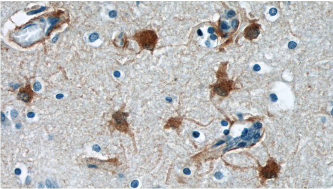
Immunohistochemical of paraffin-embedded human brain using Catalog No:114178(PRDX6 antibody) at dilution of 1:50 (under 40x lens)
